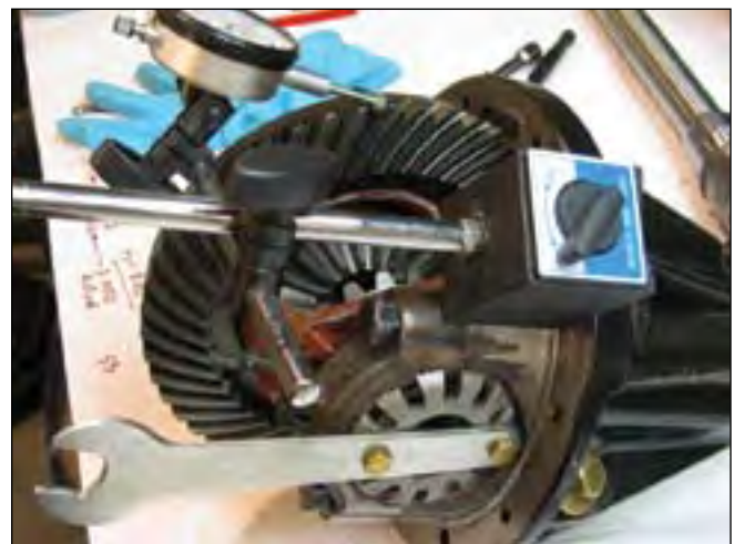
Crown-wheel back-lash adjustment with peg spanner and dial indicator
